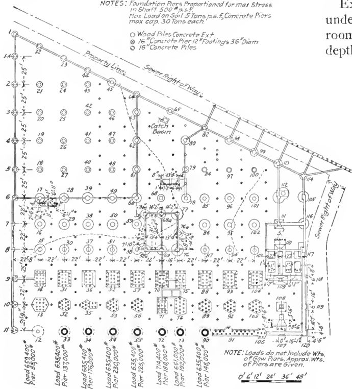
FOUNDATION LAYOUT
